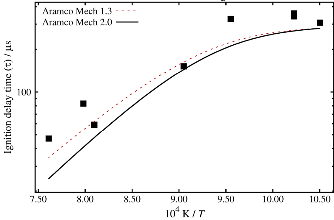
DME in Air, \Phi = 2.0 , p_{\text{average}} = 25.7 atm
