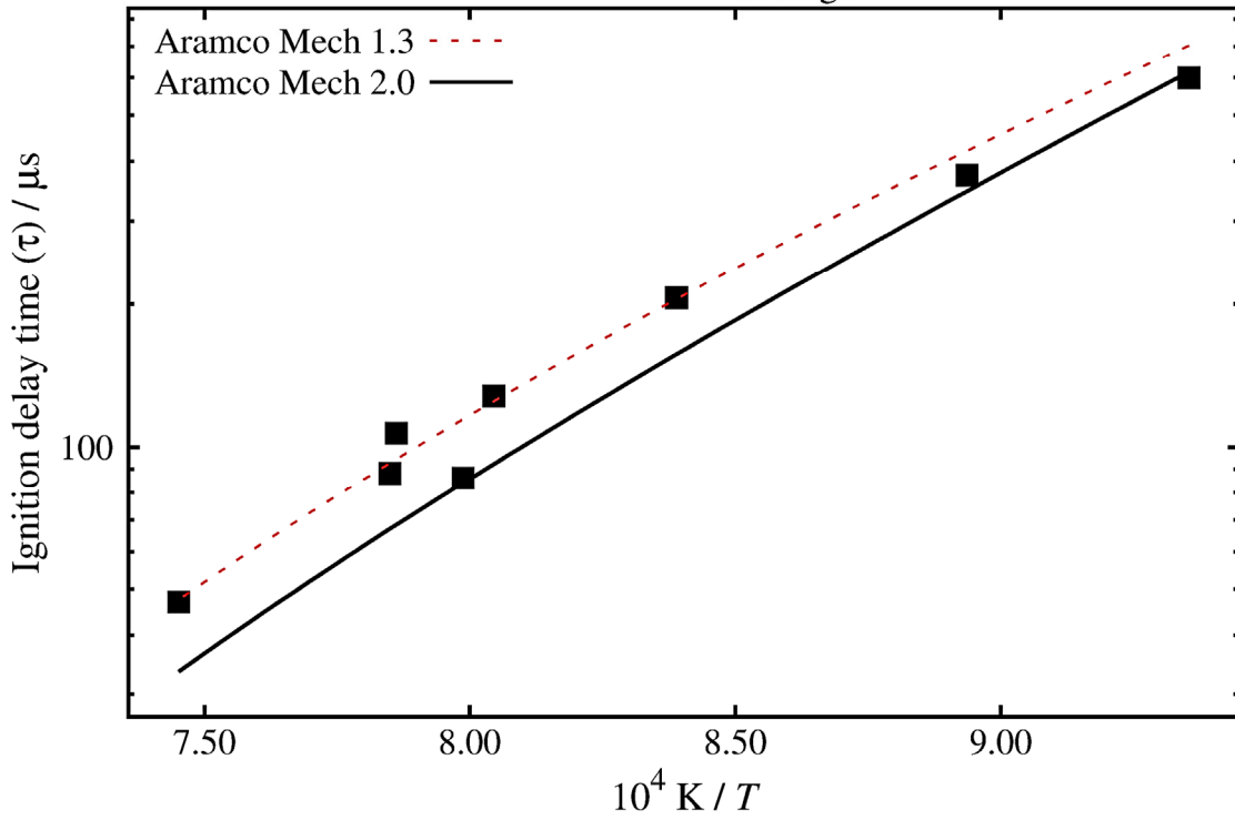
DME in Air, \Phi = 0.5 , p_{\text{average}} = 25.4 atm
