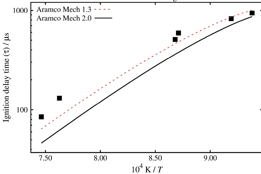
DME in Air, \Phi = 0.3 , p_{\text{average}} = 23.74 atm
