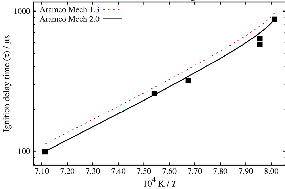
DME in Air, \Phi = 0.5 , p_{\text{average}} = 1.81 atm
