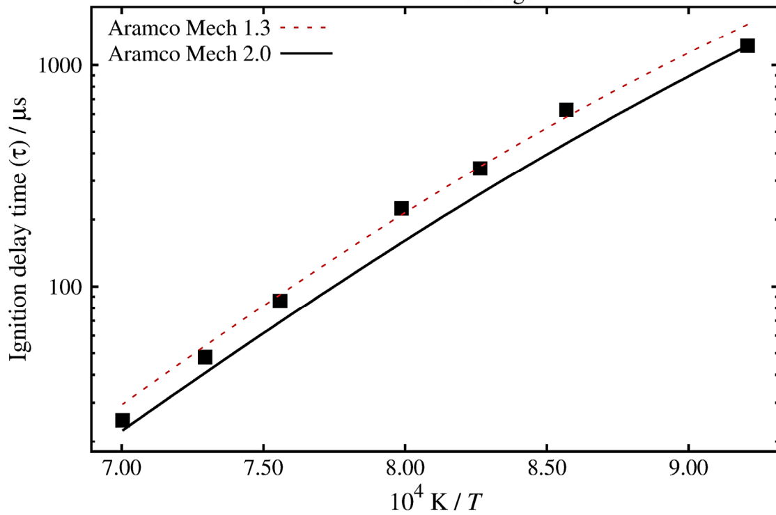
DME in Air, \Phi = 0.5 , p_{\text{average}} = 11.52 atm
