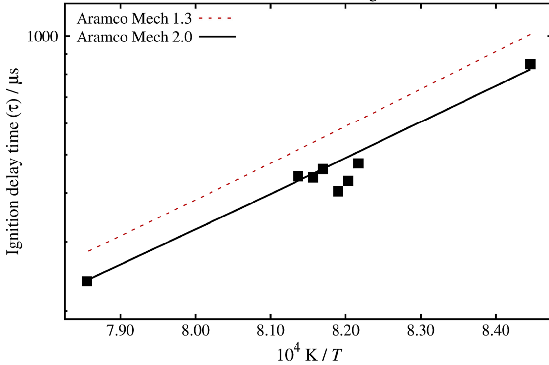
DME in Air, \Phi = 2.0 , p_{\text{average}} = 1.98 atm
