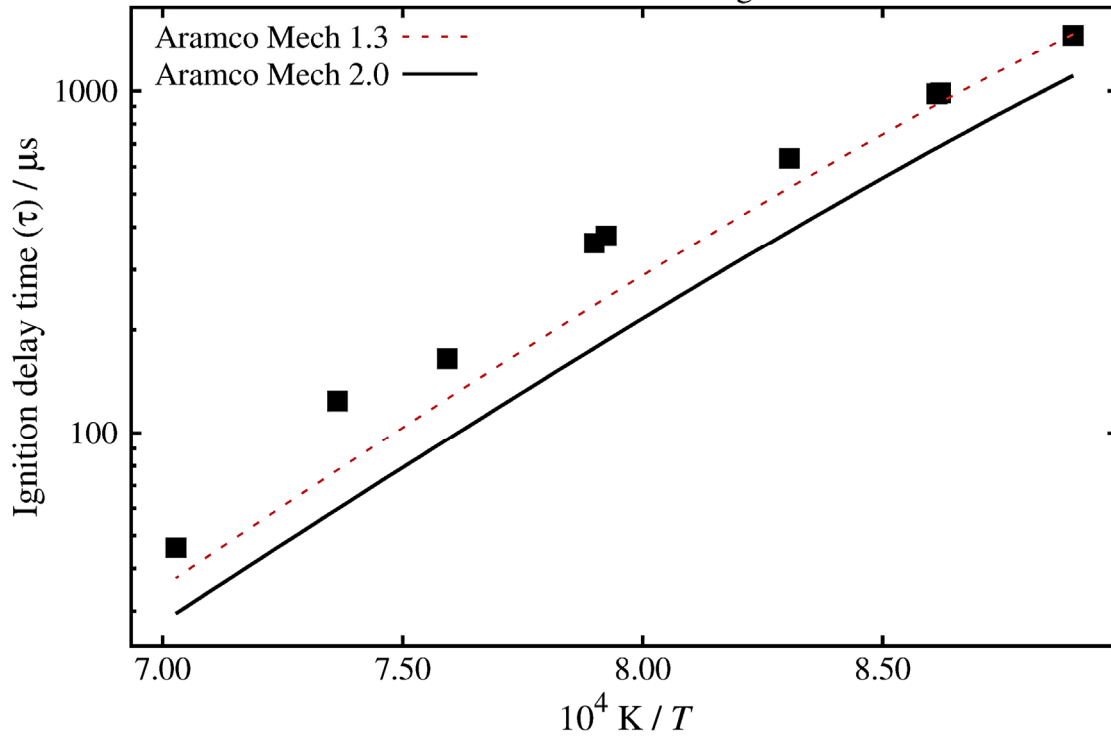
DME in Air, \Phi = 0.3 , p_{\text{average}} = 11.79 atm
