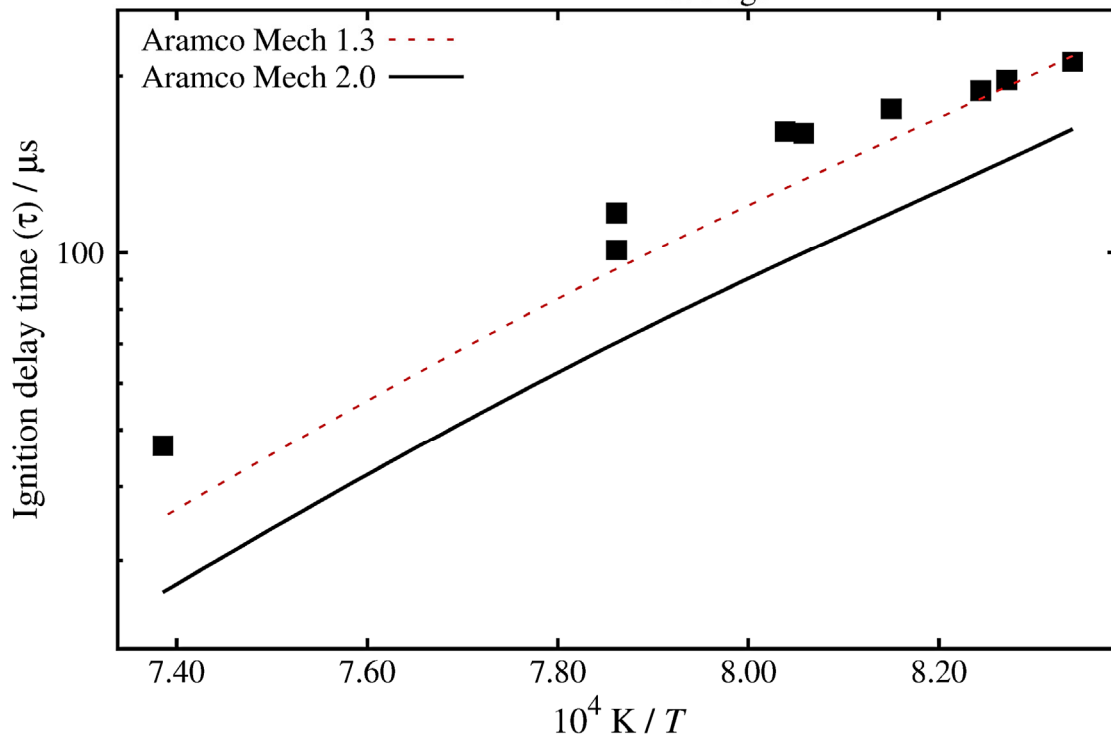
DME in Air, \Phi = 2.0 , p_{\text{average}} = 10.9 atm
