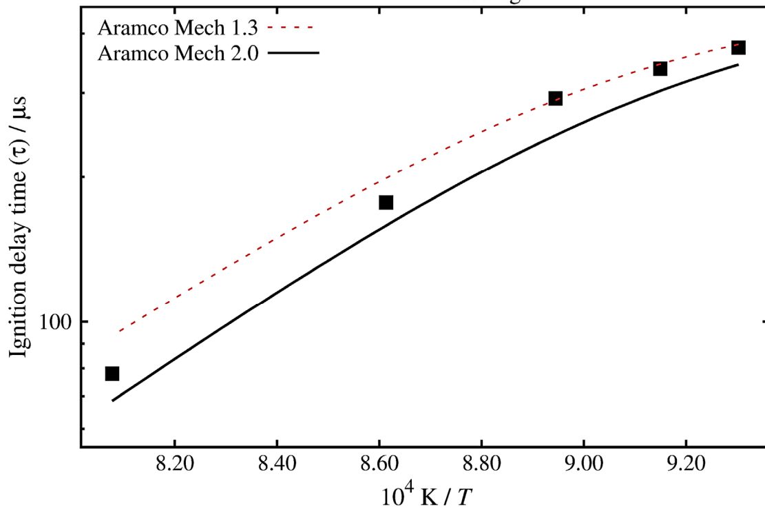
DME in Air, \Phi = 1.0 , p_{\text{average}} = 25.9 atm
