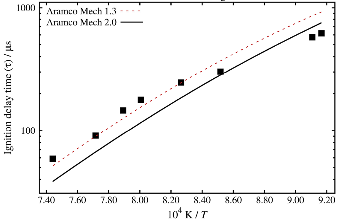
DME in Air, \Phi = 1.0 , p_{\text{average}} = 11.62 atm
