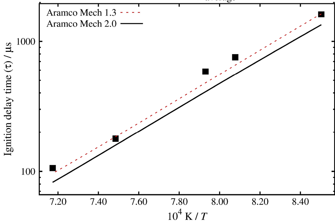
DME in Air, \Phi = 1.0 , p_{\text{average}} = 1.8 atm
