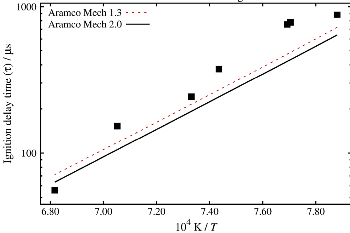
DME in Air, \Phi = 0.3 , p_{\text{average}} = 1.9 atm
